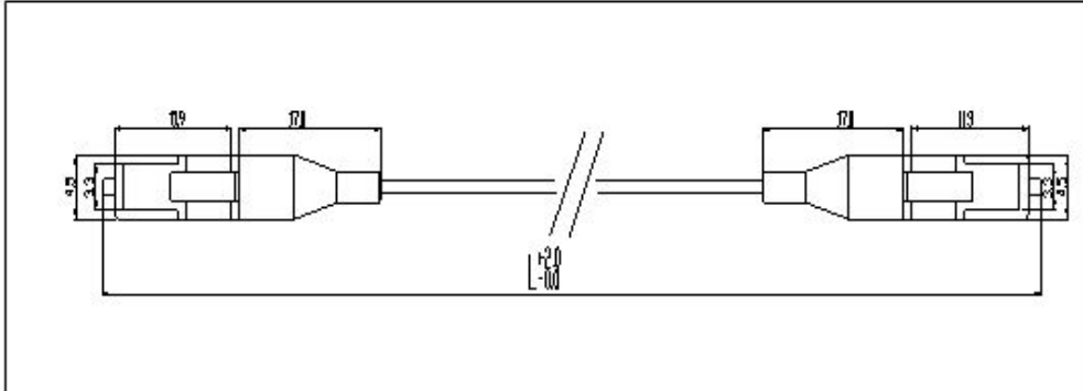
Figure1. LC 0.9 Patch Cord
